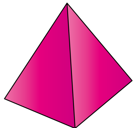
triangle pyramid
