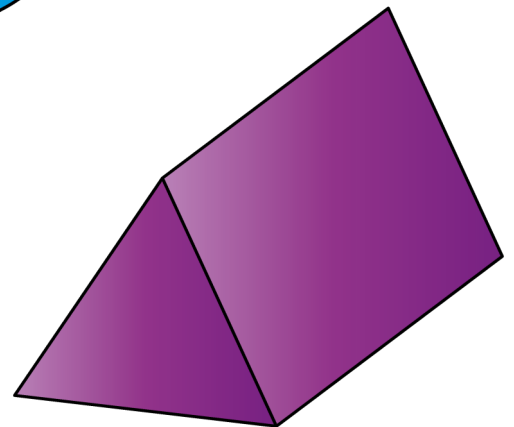
triangular prism
