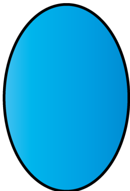
oval
