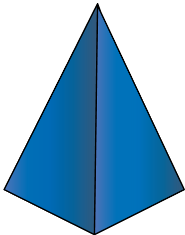
square pyramid
