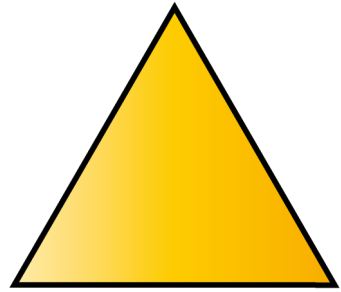
triangle
